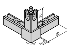
2240083 Corner joint, 3-sided, with adjustable foot
