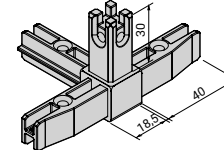
2240076 Corner joint, 4-sided
