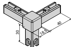
2240074 Corner joint, 3-sided
