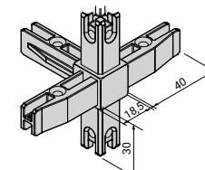
2240077 Corner joint, 5-sided
