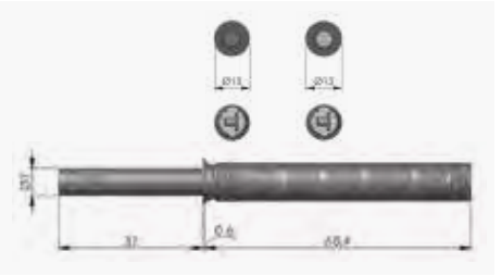
Kpush Auswerfer, anthrazit, l=37 mm
